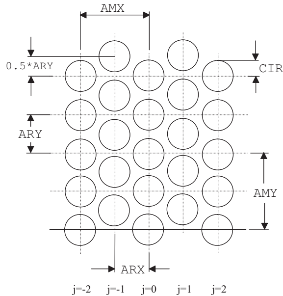
Figure 8.37: Hexagonal arrangement of array cells. All odd numbered columns are shifted (staggered) in Y-direction by 0.5 \cdot \text{ARY} . Optimal packaging of cells is then accomplished with \text{ARX} = \cos(30^\circ) \cdot \text{ARY} = 0.866 \cdot \text{ARY} .
