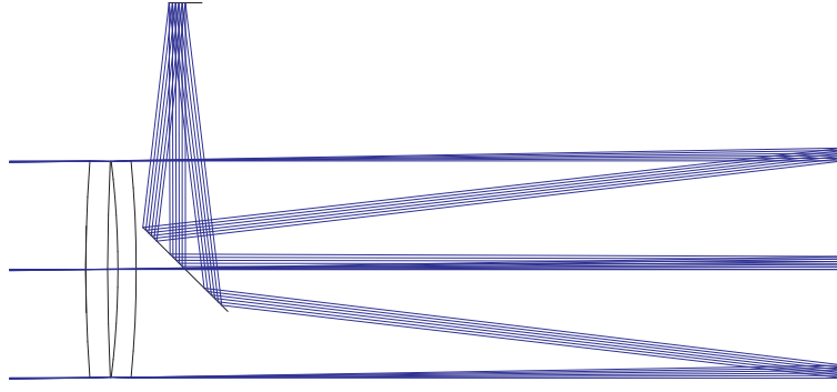
Figure 12.6: Lurie-Houghton design form.
