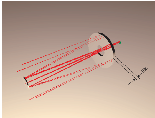
Figure 12.3: Specifying the mirror thickness THM at reflective surfaces
