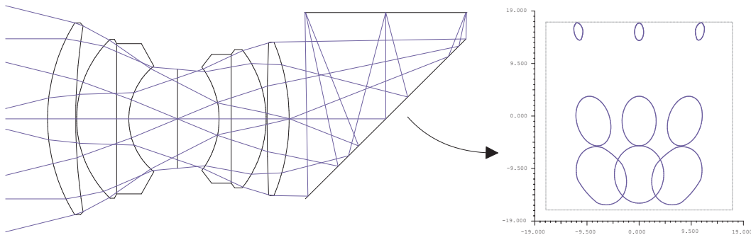
Figure 23.1: Beam footprints on fold mirror behind a Double Gauss lens. The corresponding example file can be found in $i\examples\misc\DOUBLE_GAUSS-2_fold_mirr .
