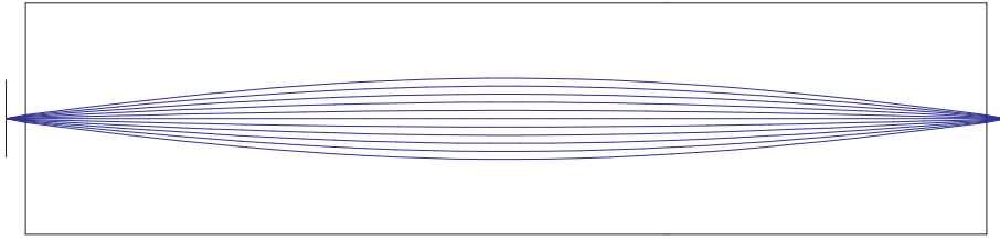
Figure 14.34: Coupling of two Corning SMF28 fibers with NSG-SELFOC TM lens SLW10.
