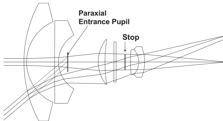
Figure 7.8: Ray aiming methods. Rays aiming to the paraxial entrance pupil (RAIM ENP) will not hit the stop surface at the corresponding coordinates. RAIM ST0 takes account for pupil aberrations in centered and decentered systems by iterating for the exact start coordinates.
