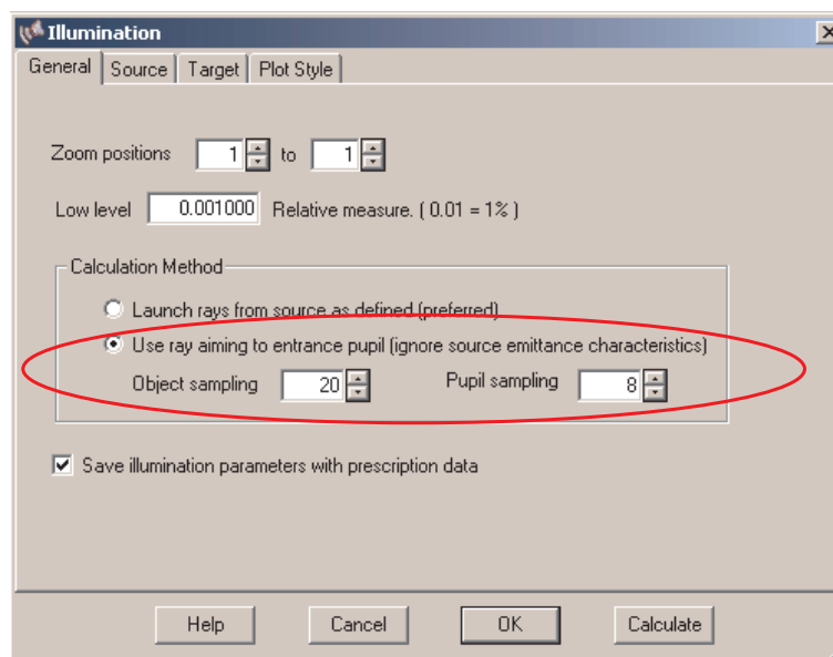
Figure 15.10: Selecting alternative illumination option: Aiming source rays to the entrance pupil directly. The number of rays traced per source is (objectsampling)^2 \cdot (pupilsampling)^2 \cdot NumberOfColours
