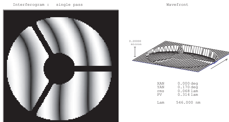
Figure 14.27: Interferogram, computed from wavefront aberration at one discrete field point.
