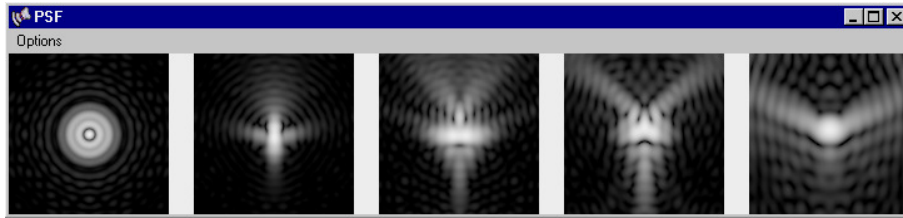
Figure 14.21: Diagonal field PSF as gray-coded bitmaps, using the PSF DF command.
