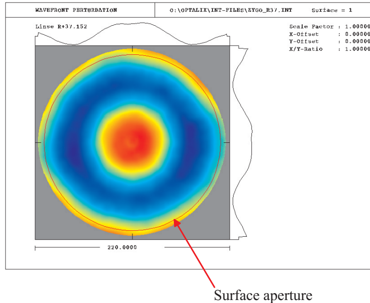
Figure 8.43: Display interferogram deformation on a surface. The corresponding example file can be found in the $i\examples\Misc\Simple_Achromat_INT_Deformation.otx . The surface aperture is shown in red colour which allows a direct comparison with the measured interferogram dimensions.
