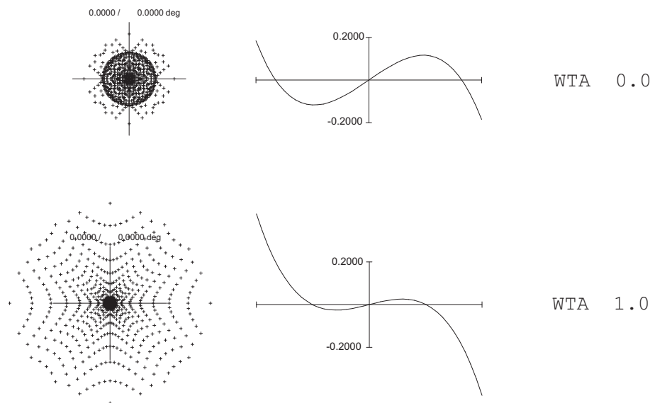
Figure 19.7: Effect of 'weight on aperture' (WTA) on spot shape (left) and transverse aberrations (right), by minimizing spot diameter (e.g. spd f1 @ ). High values emphasize the central core of the spots at the expense of a larger blur.
