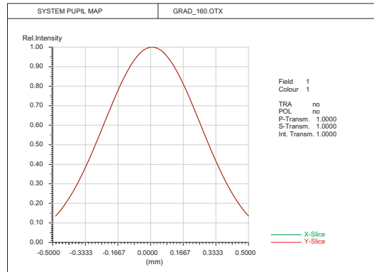
Figure 14.6: Pupil intensity maps shown by XY-slices (XY) representations.
