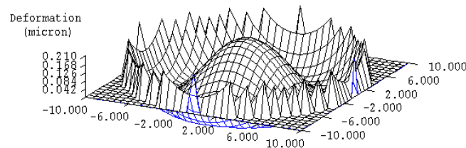
Figure 8.44: Fringe Zernike deformation, using only coefficient 9.
