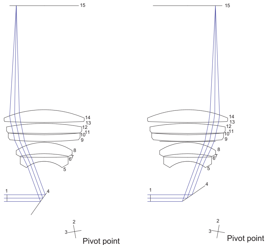
Figure 8.31: Use of global coordinates and NOR surfaces for modelling of a polygon scanner.
