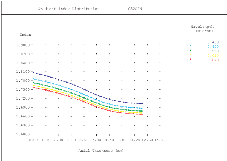
Figure 24.6: Gradient index profile, shown for five wavelengths.
