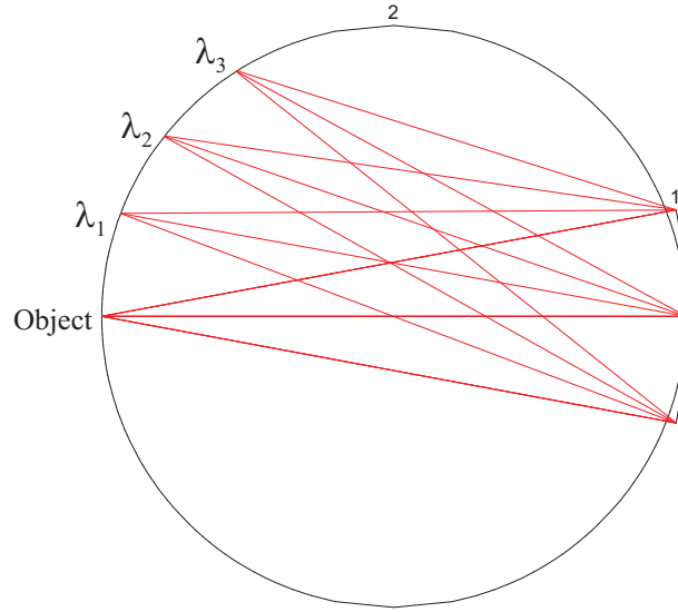
Figure 8.16: Rowland grating.
