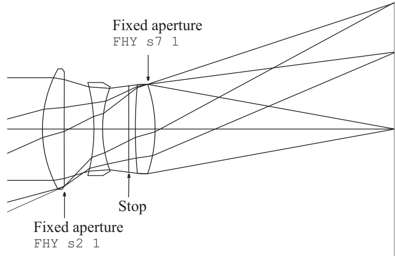
Figure 8.51: Defining vignetting characteristics with fixed apertures.
