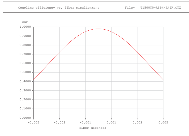
Figure 12.5: Example output of user defined graphics: CEF vs. fiber misalignment.
