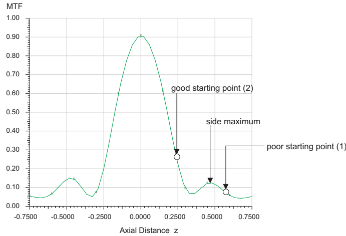
Figure 19.10: Variation of diffraction MTF for a perfect lens as a function of defocus.
