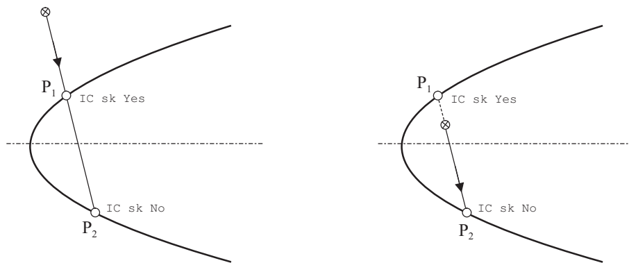
Figure 8.10: Selection of alternate intersection point and geometrical meaning of IC code. Left: ray starting 'outside' surface, right: ray starting 'inside' surface.
