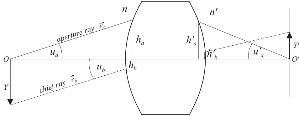
Figure 5.6: Definition of paraxial entities.
