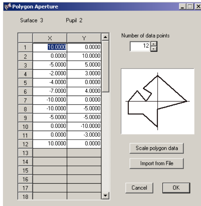
Figure 8.48: Dialog-based editing of polygon apertures.
