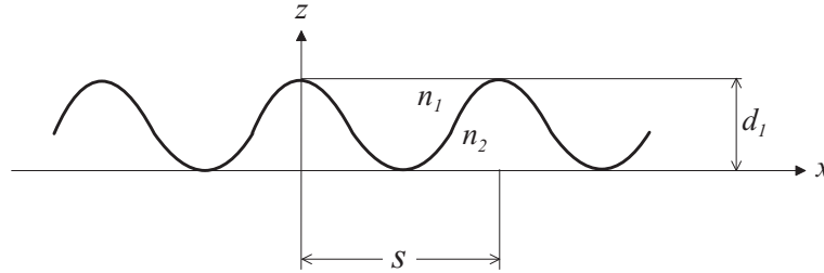
Figure 8.14: Sinusoidal profile of a diffracting structure.
