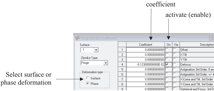
Figure 8.46: Editing of Zernike phase coefficients.
