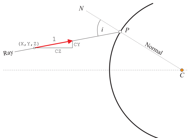
Figure 5.5: Definition of rays.
