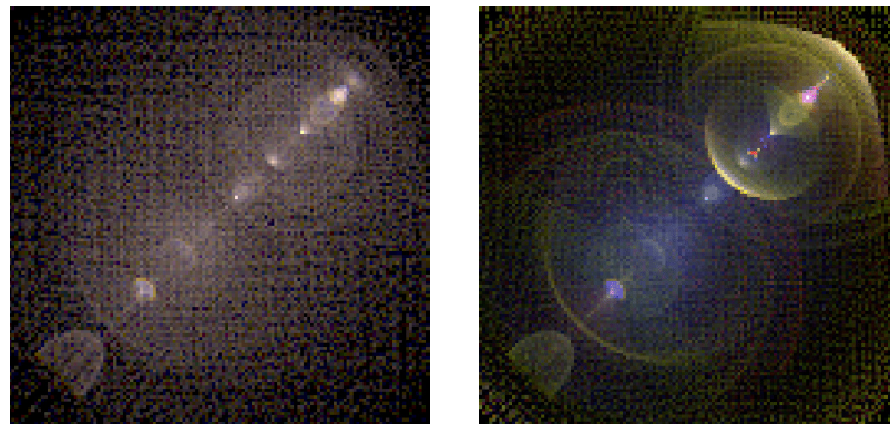
Figure 14.12: Almost photo-realistic rendering of ghost effects as a RGB-image on the example of $i\examples\high_na\f15_33_ghost.otx . The left image was obtained by ignoring coating or Fresnel reflection effects, whereas the right image is more realistic by including coating effects (POL Y, TRA Y)
