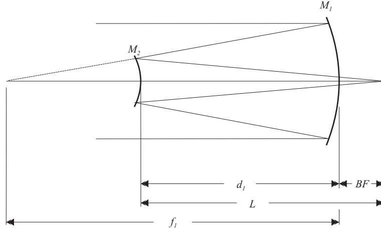
Figure 12.7: Paraxial quantities at a compound telescope
