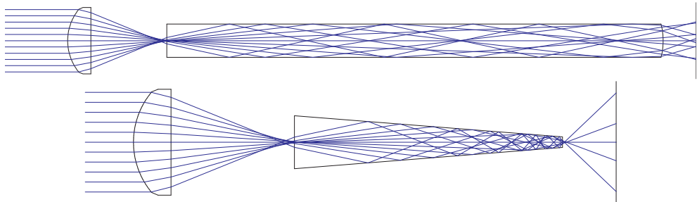
Figure 8.34: Light pipe (top) and tapered fiber (bottom). The corresponding example files can be found in the $i\examples\LightPipe directory as LIGHTPIPE1.OTX , TAPERED_FIBER.OTX .
