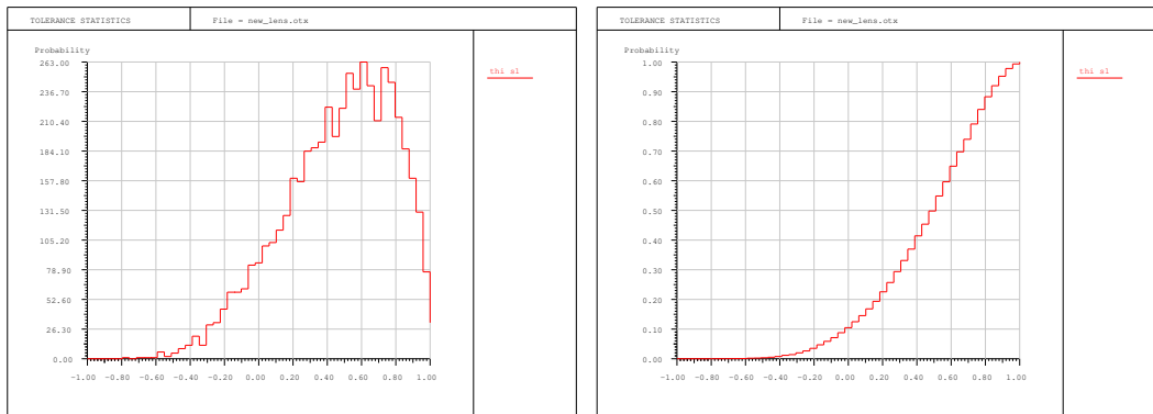
Figure 22.6: Beta distribution. Left: linear plot, right: cumulative plot.
