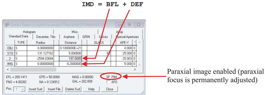
Figure 7.7: Display of image distance (IMD) and defocus (DEF) in the surface editor.
