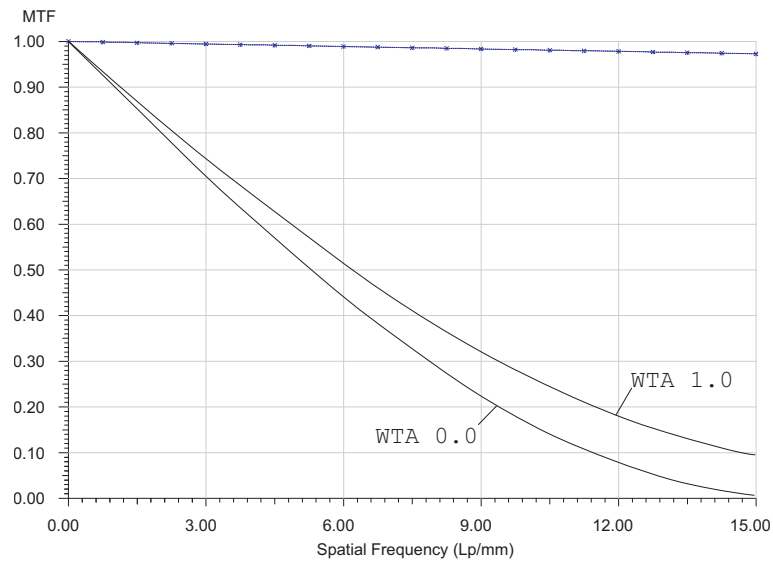
Figure 19.8: Effect of 'weight on aperture' (WTA) setting on MTF. High values improve the high-frequency components of MTF (i.e. high resolution), low values improve the low-frequency components of MTF (i.e. high contrast). Note that the curves above only show the case of improving high-frequency components.
