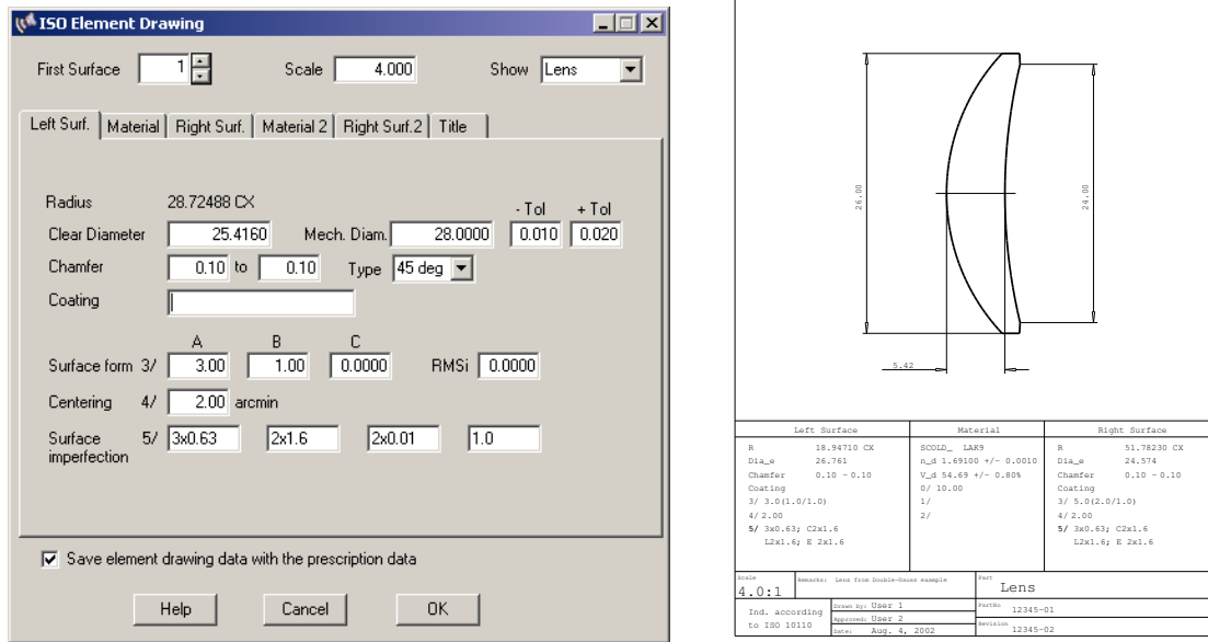
Figure 23.7: ISO element drawing dialog box for editing element drawing indications (left) and corresponding sample output (right). The dialog box is invoked from the command line by the command ELE ?.
