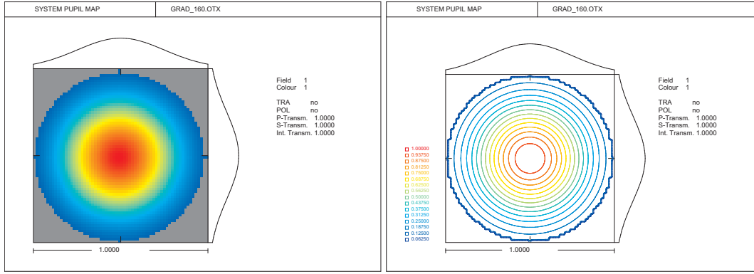
Figure 14.5: Pupil intensity maps shown in false-colour (FAL) and contour (CON) representations.
